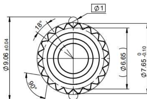
DETAIL D Teeth Z=20
