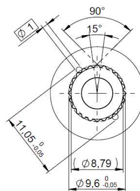
MILLING DETAIL 24 Teeth DETAIL 2 : 1
